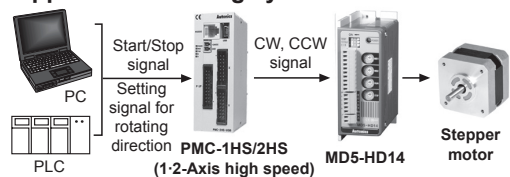
PMC-1HS/2HS (1/2-Axis high speed) PMC-2HSP/2HSN (2-Axis high speed Interpolation Normal) PMC-4B-PCI (4-Axis board type)
